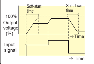
Soft-start & Soft-down action diagram
