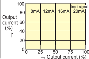
Constant current control characteristic diagram
