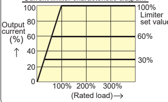
Current limiter characteristic diagram
