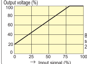
Base-up output characteristic diagram
