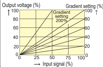
Gradient setting output characteristic diagram
