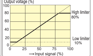
High & Low limiter characteristic diagram
