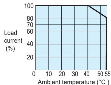
• Temperature characteristics of load current
