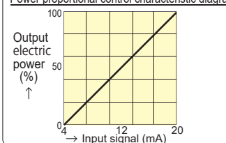
Power proportional control characteristic diagram
