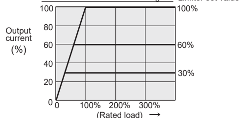
Current limiter characteristic diagram
